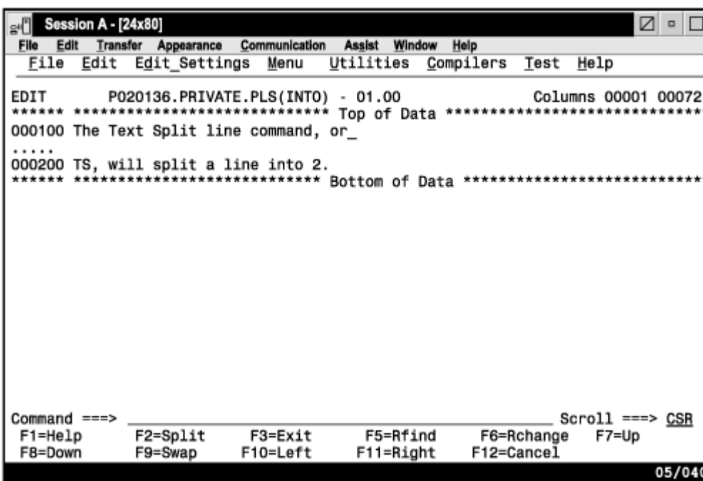
Figure 104. After TS (Text Split) line command
