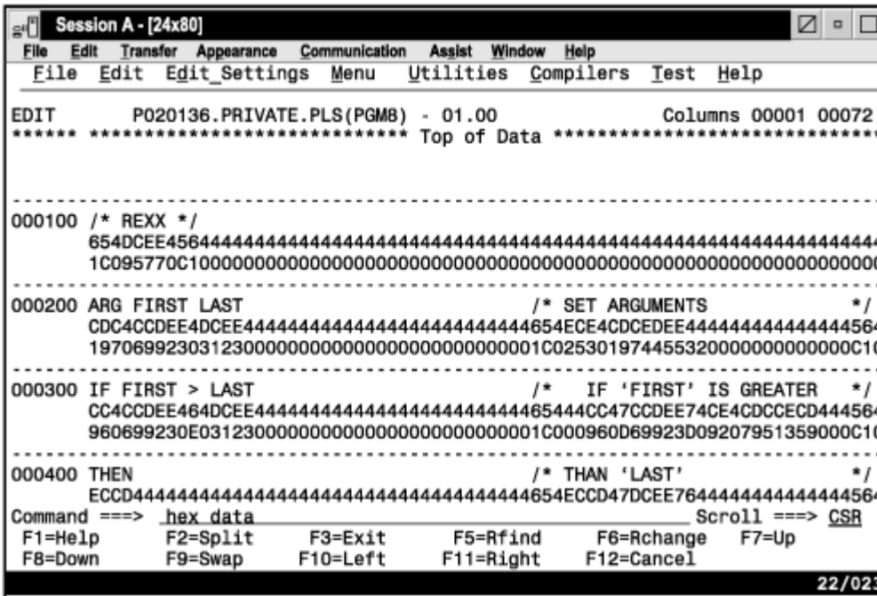
Figure 128. Hexadecimal display, vertical representation
