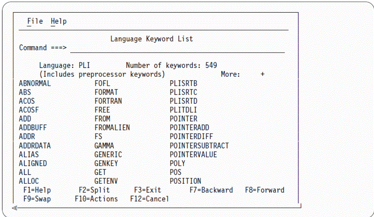
Figure 8. HILITE Language Keyword List (ISREPK)
